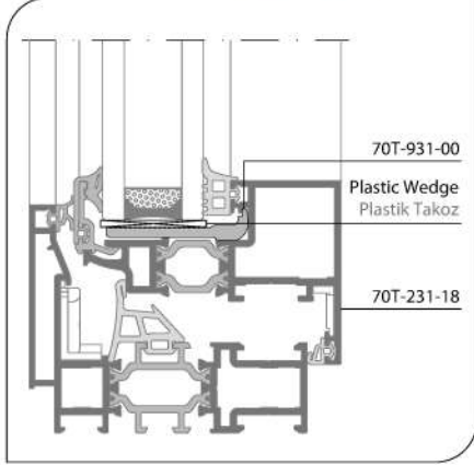
SECTION / KESİT
