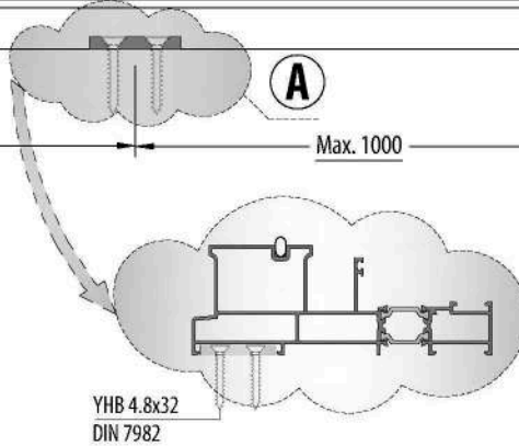
A DETAIL DETAYI
