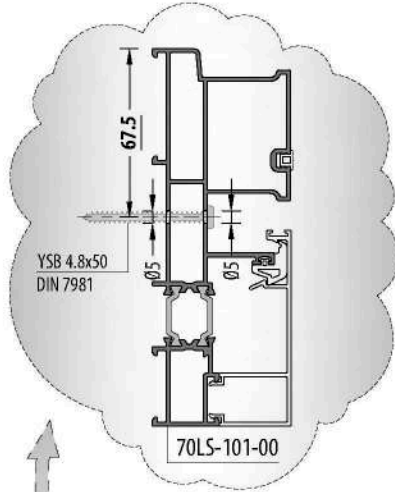
B DETAIL / DETAYI
